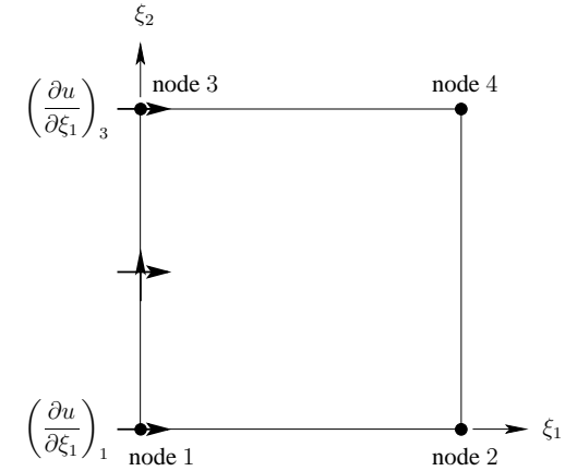
FIGURE 1.13: Interpolation of nodal derivative \frac{\partial u}{\partial \xi_1} along side 1–3 of a bicubic Hermite element.
