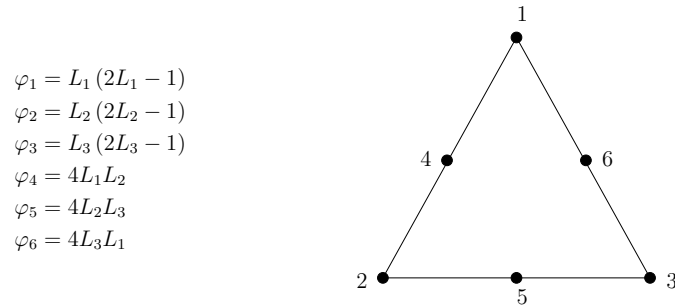
FIGURE 1.16: Basis functions for a six node quadratic triangular element.
