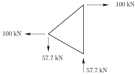
FIGURE 5.3: Reaction forces for the truss system of Figure 5.2.
