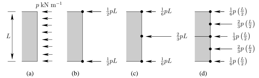
FIGURE 5.4: A uniform boundary stress applied to the element side in (a) is equivalent to nodal loads of \frac{1}{2}pL and \frac{1}{2}pL for the linear basis used in (b) and to \frac{1}{6}pL , \frac{2}{3}pL and \frac{1}{6}pL for the quadratic basis used in (c). Two adjacent quadratic elements both contribute to a common node in (d), where the element length is now \frac{L}{2} .
