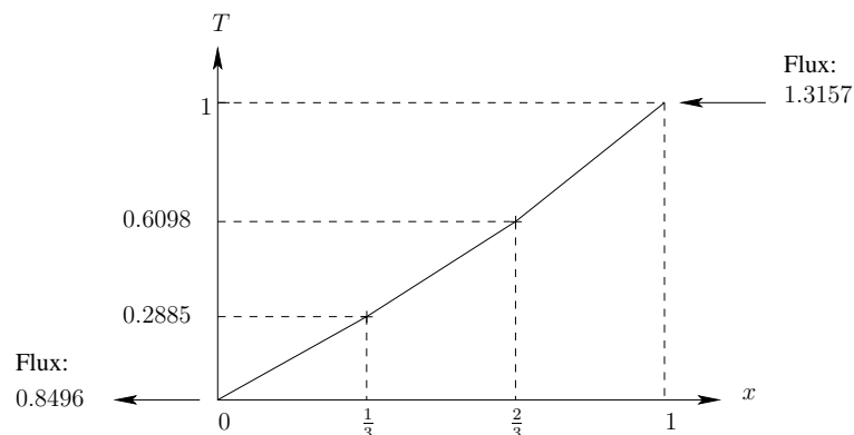
FIGURE 2.2: Finite element solution of one-dimensional heat equation.
