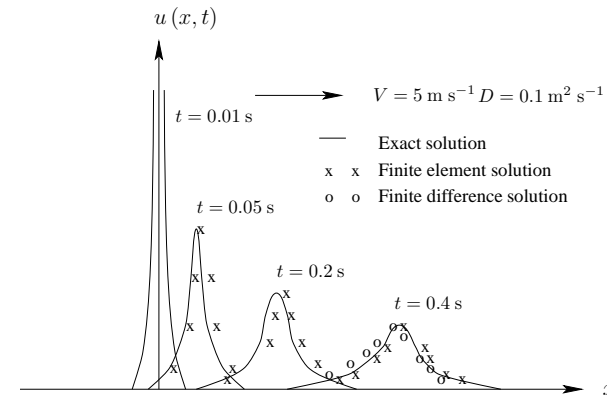
FIGURE 4.4: Advection-diffusion of a unit mass pulse. The finite element solutions (at t=0.01 s, 0.05 s, 0.2 s and 0.4 s) and finite difference solutions (at t=0.4 s only) are compared with the exact solution. \Delta x=0.1, \Delta t = 0.001 s for 0 < t < 0.01 s and \Delta t = 0.01 for t \geq 0.01 s.
