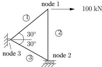
FIGURE 5.2: A system of three trusses.
