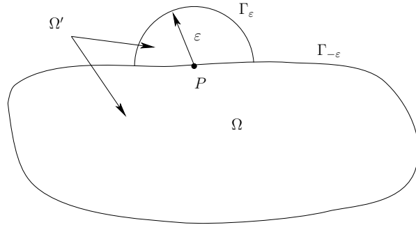
FIGURE 5.5: Illustration of enlarged domain when singular point is on the boundary.
