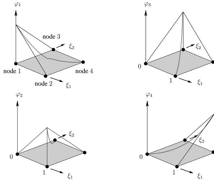
FIGURE 1.9: Two-dimensional bilinear basis functions.
