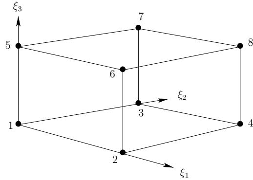
FIGURE 1.11: An 8-node trilinear element.
