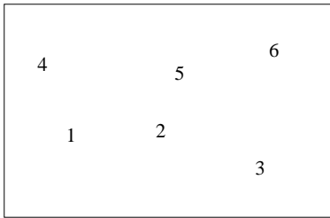
FIGURE 1.20: Node positions for example 111.
