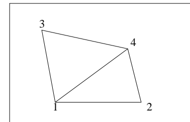
FIGURE 1.24: Defining a triangular mesh for example 116
