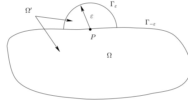
FIGURE 3.3: Illustration of enlarged domain when singular point is on the boundary.
