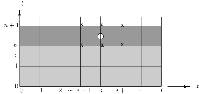
FIGURE 4.2: An implicit finite difference scheme based on central differences in t , as well as x , which tie together the 6 points shown by x . The equation is centred at the point (i, n + \frac{1}{2}) shown by the O . The lightly shaded region shows where the solution is known at time step n . The dark shading shows the region of the coupled equations.
