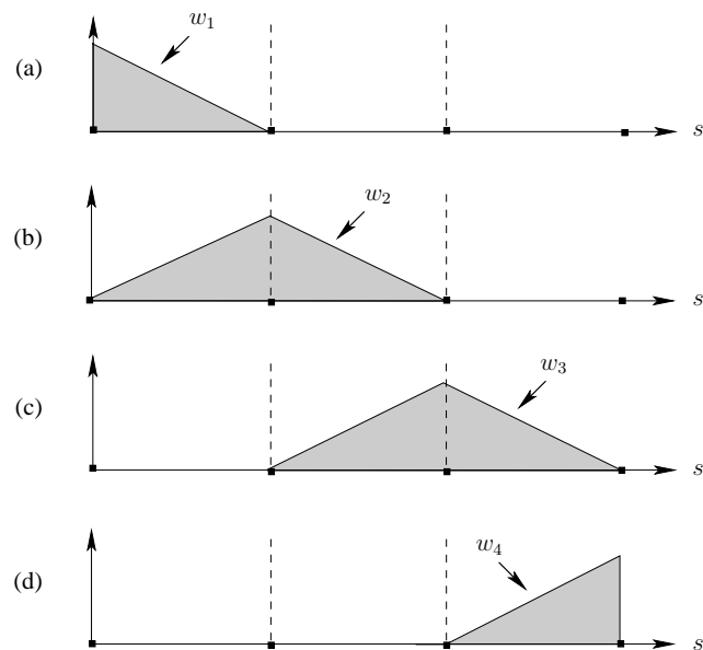
FIGURE 1.6: (a) . . . (d) The weighting functions w_n associated with the global nodes n = 1 \dots 4 , respectively. Notice the linear fall off in the elements adjacent to a node. Outside the immediately adjacent elements, the weighting functions are defined to be zero.
