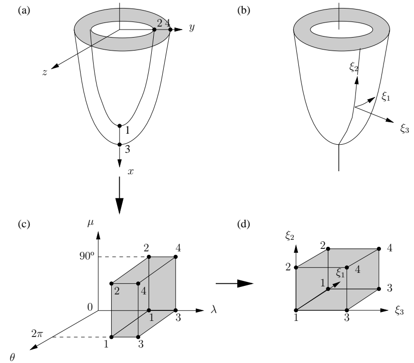
FIGURE 1.19: A single prolate spheroidal element, shown (a) in (x, y, z) -coordinates, (c) in (\lambda, \mu, \theta) -coordinates and (d) in (\xi_1, \xi_2, \xi_3) -coordinates, (b) shows the orientation of the \xi_i -coordinates on the prolate spheroid.
