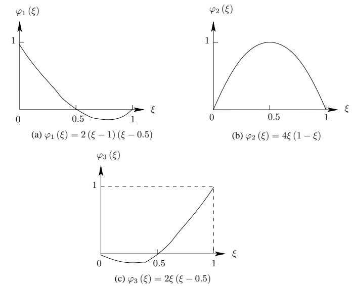
FIGURE 1.8: One-dimensional quadratic basis functions.
