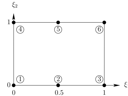
FIGURE 1.10: A 6-node quadratic-linear element (node numbers circled).
