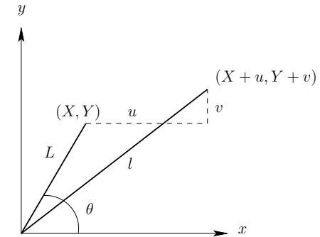
FIGURE 5.1: A truss of initial length L is stretched to a new length l . Displacements of the right hand end relative to the left hand end are u and v in the x - and y -directions, respectively.
