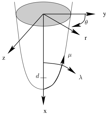
FIGURE 1.18: Prolate spheroidal coordinates.
