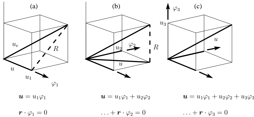
FIGURE 2.3: Showing how the Galerkin method maintains orthogonality between the residual vector \mathbf{r} and the set of basis vectors \varphi_i as i is increased from (a) 1 to (b) 2 to (c) 3.
