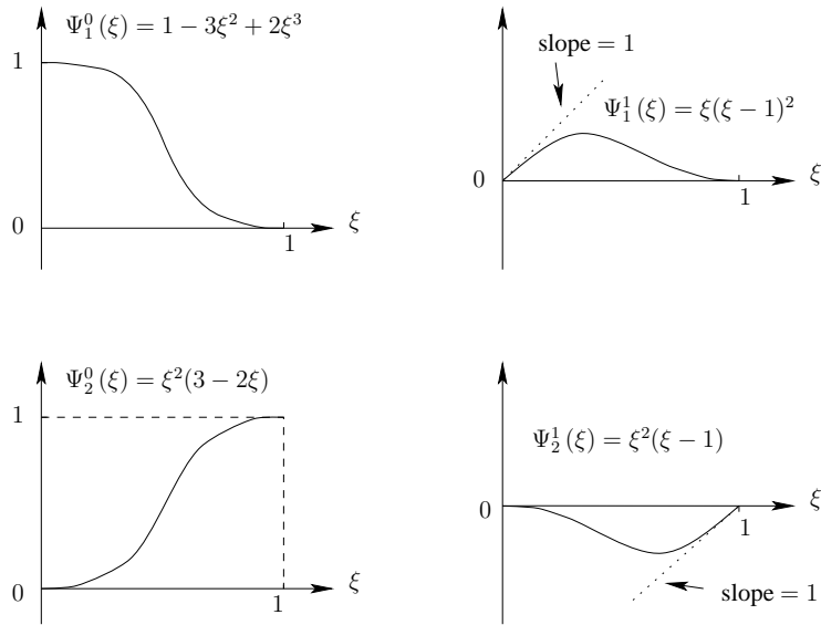
FIGURE 1.12: Cubic Hermite basis functions.
