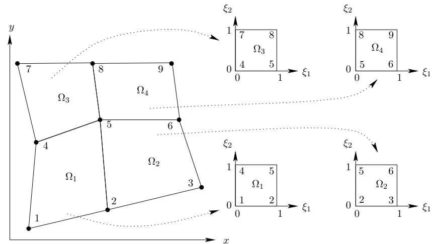
FIGURE 2.5: Mapping each \Omega to the \xi_1, \xi_2 plane in a 2 \times 2 element plane.
