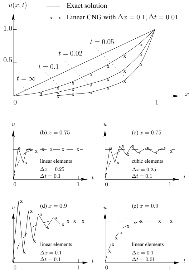
FIGURE 4.3: Analytical and numerical solutions of the transient 1D heat equation showing the effects of element size \Delta x and time step size \Delta t . The top graph shows the exact and approximate solutions as functions of x at various times. The lower graphs show the solution through time at the specified x positions and with various choices of \Delta x and \Delta t as indicated.
