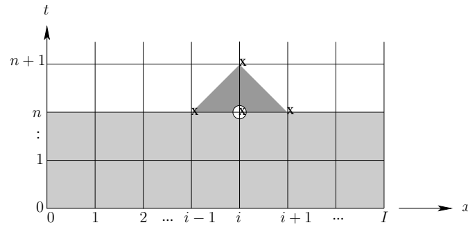
FIGURE 4.1: A finite difference grid for the solution of the transient 1D heat equation. The equation is centred at grid point (i, n) shown by the O . The lightly shaded region shows where the solution is known at time step n . With central differences in x and a forward difference in t an explicit finite difference formula gives the solution at time step n + 1 explicitly in terms of the solution at the three points below it at step n , as indicated by the dark shading.
