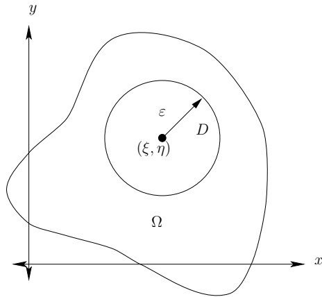
FIGURE 3.2: Domain used to evaluate fundamental solution coefficients.
