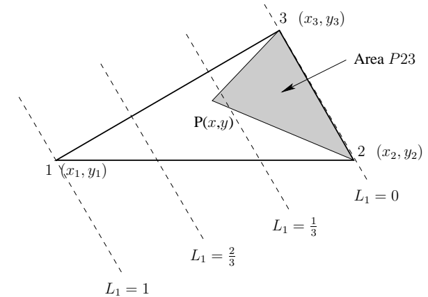
FIGURE 1.15: Area coordinates for a triangular element.
