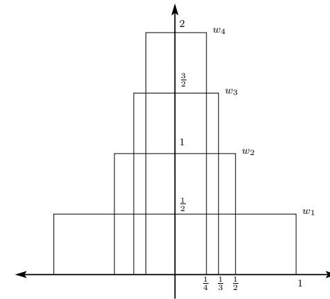
FIGURE 3.1: Illustrations of unit force distributions w_n .
